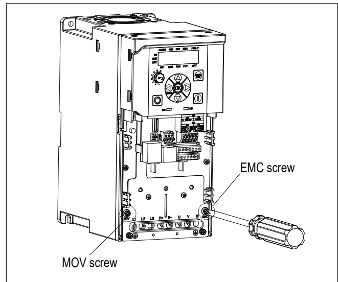
Figure 6. Location of the EMC/MOV screws in frames 2-4.
