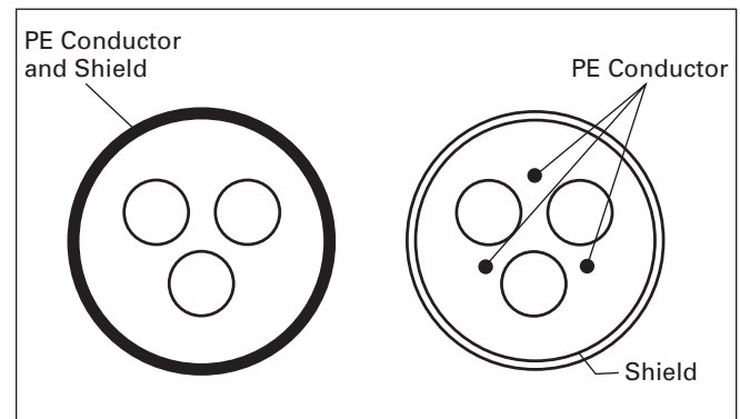
Figure 9. Cable description.
