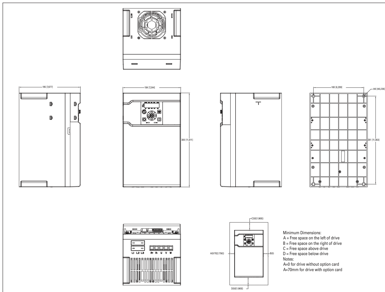
Figure 18. DM1 Pro FR4 without NEMA 1 kit dimension drawing.
