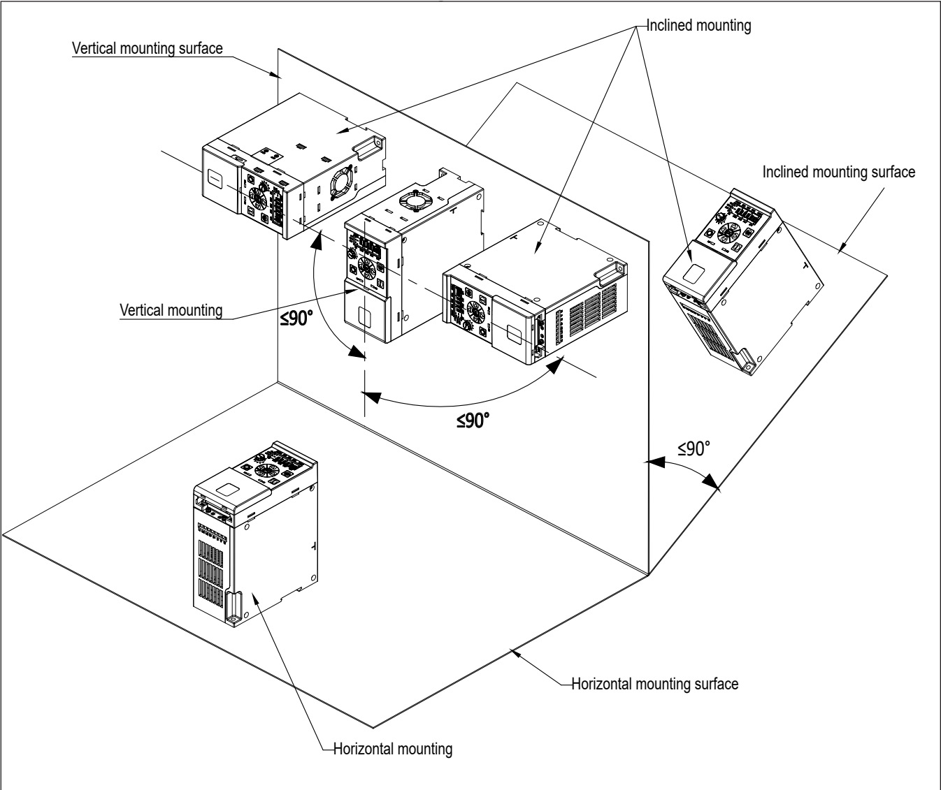
Figure 7. Mounting orientation.
