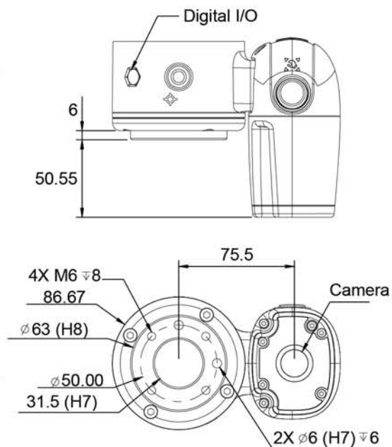
Camera Flange
