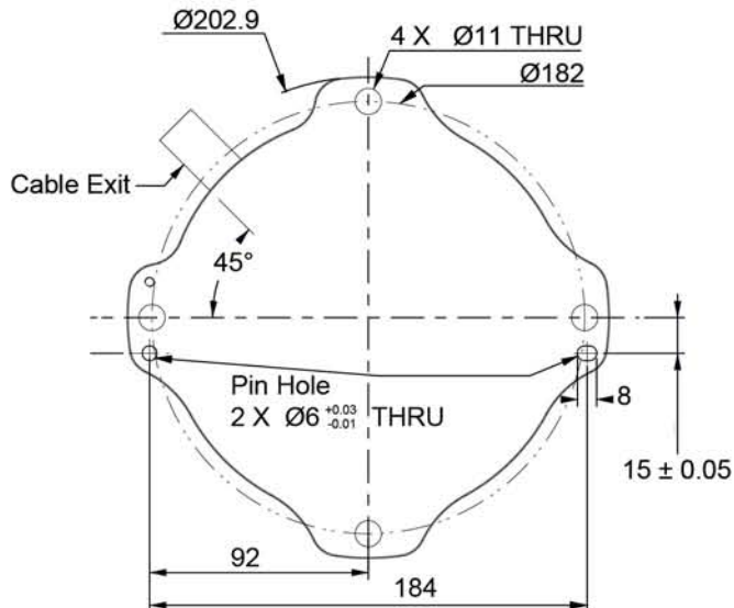
Camera Flange
