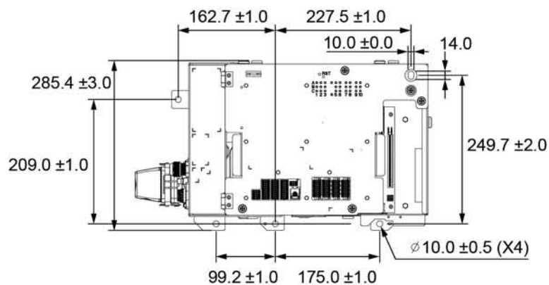
Control Box (DC)
