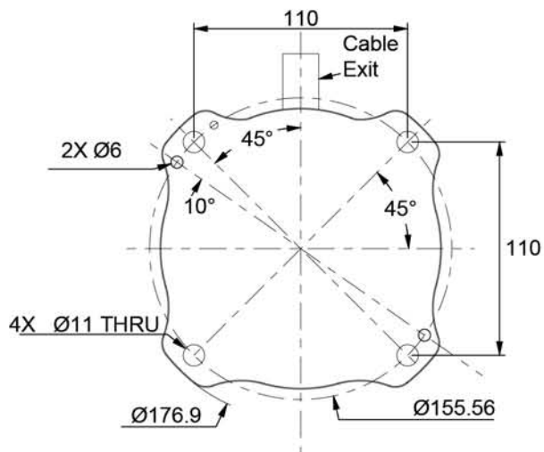
Footprint (TM5S/7S Models)
