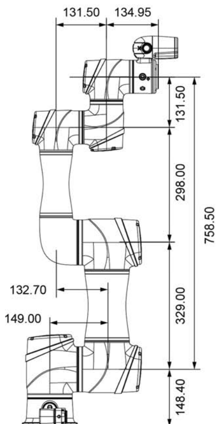
TM7S/TM7S-X/TM7S-M *
