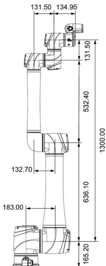
TM12S/TM12S-X/TM12S-M *
